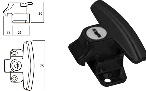
Lockable body
