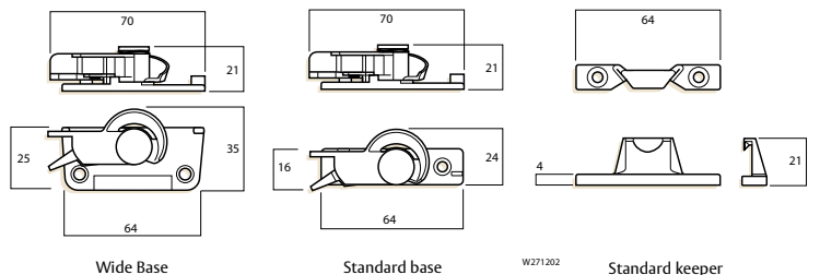
Wide Base
